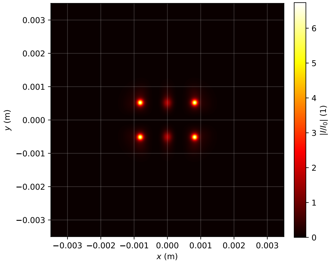
Intensity profile I(x, y, z = 0.398)/I_0 , P_{in}=9.0P_{cr} , artificial time
